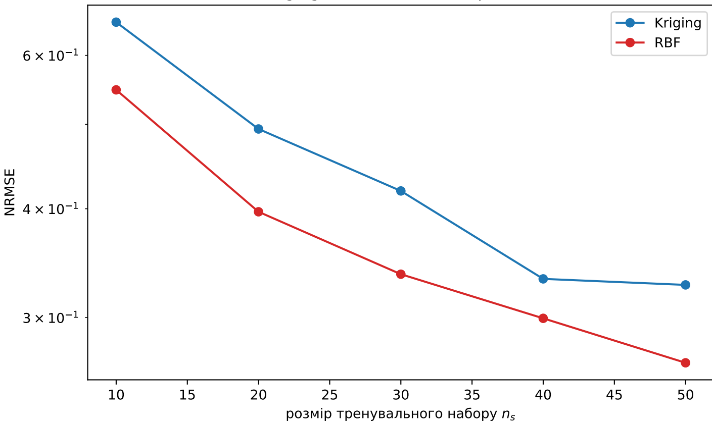
RBF vs Kriging на Heat-AMIcon / q (LHS-дизайн)
